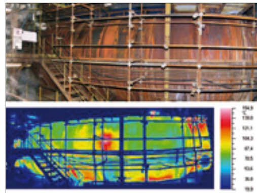
▲ Infrared thermal image of a damage furnace
