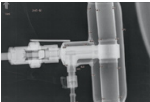
▲ Computerized radiographic image
