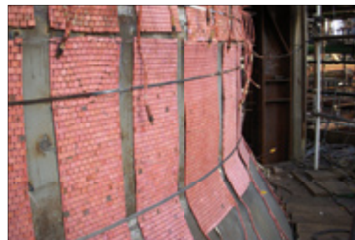
▲ Post weld heat treatment preparation of a circumferential weld of a column
